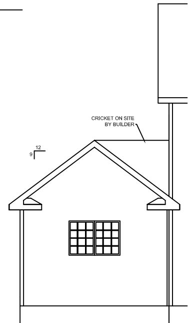
FRONT ELEVATION
